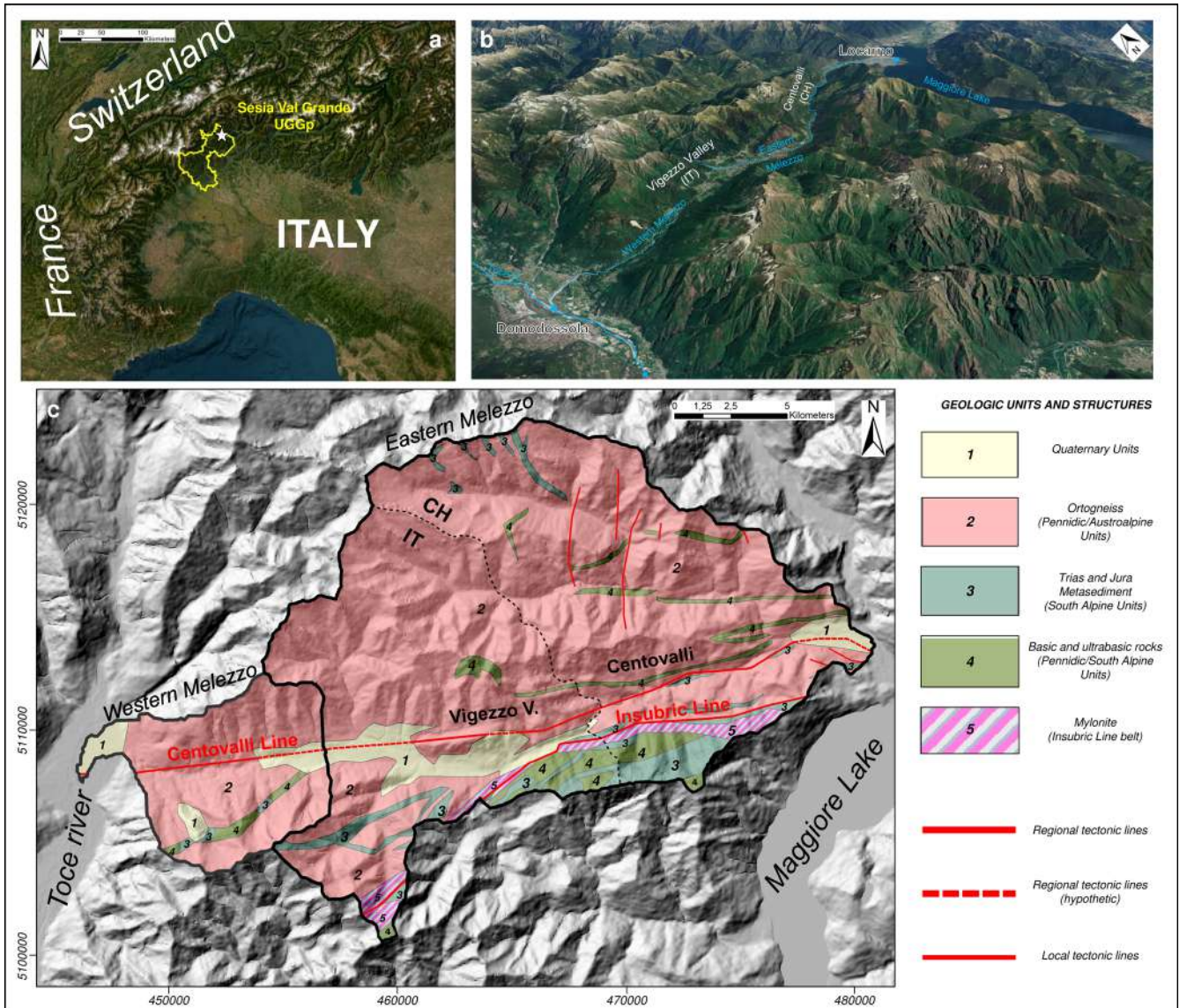
Figure 1 - The Vigezzo Valley location. a) location in Northern Italy, within the Sesia Val Grande UNESCO Global Geopark; b) 3D view of the Melezos hydrographic basin (Google Earth); c) geological map of the area derived from the Swiss geological map (1:500,000; source: swisstopo service), drawn on the hillshade (source: Geoportale Regione Piemonte), with the Eastern and Western Melezos hydrographic basins. Coordinate system is WGS 1984 UTM, Zone 32.
